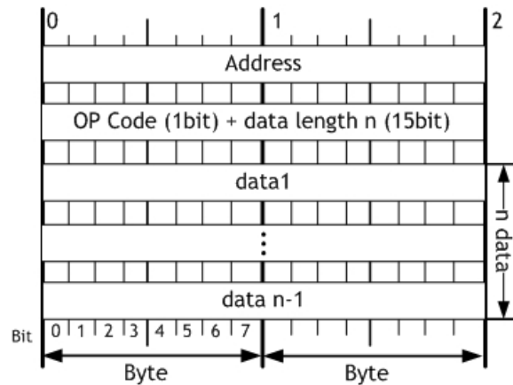
Figure 19 W5200 SPI Frame Format
