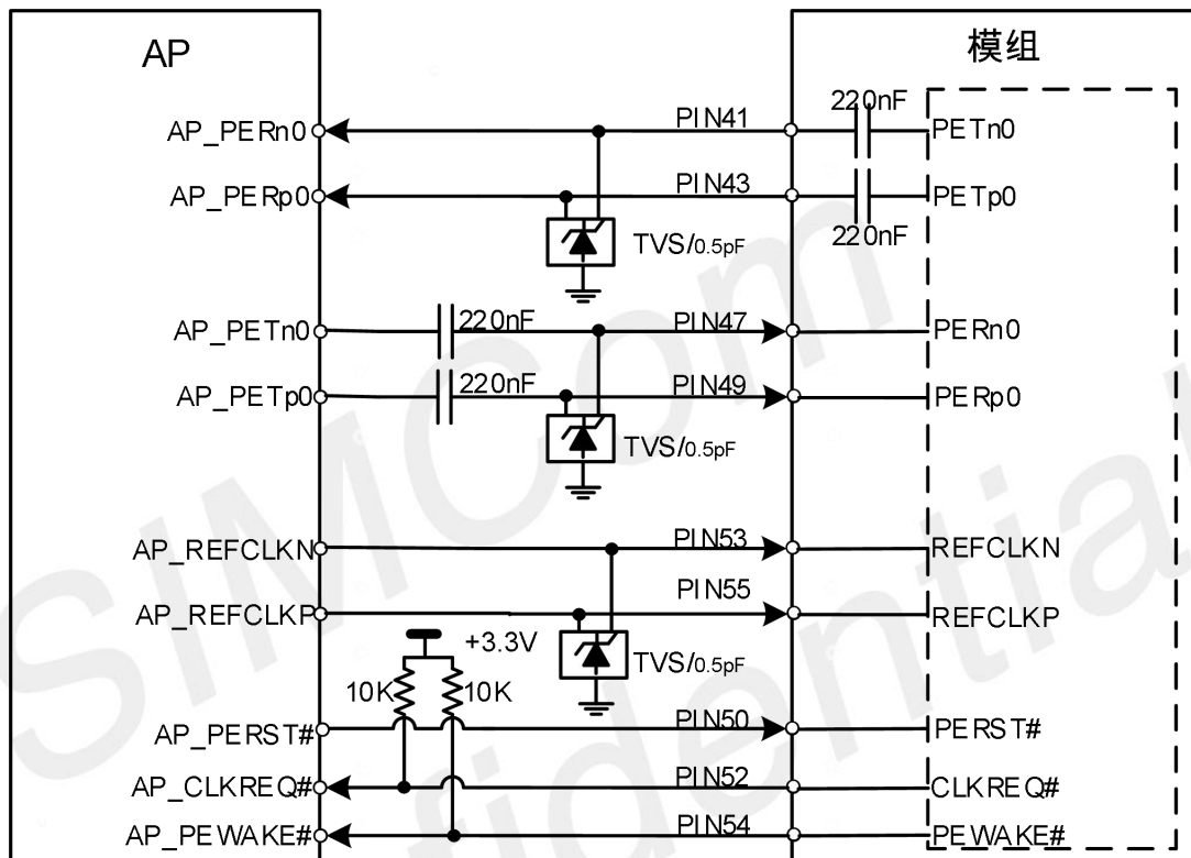
Figure 22: PCIe interface reference circuit (EP Mode)
