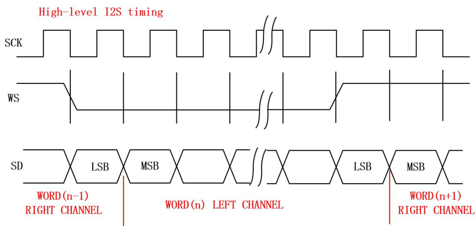
Figure 29: I2S timing
