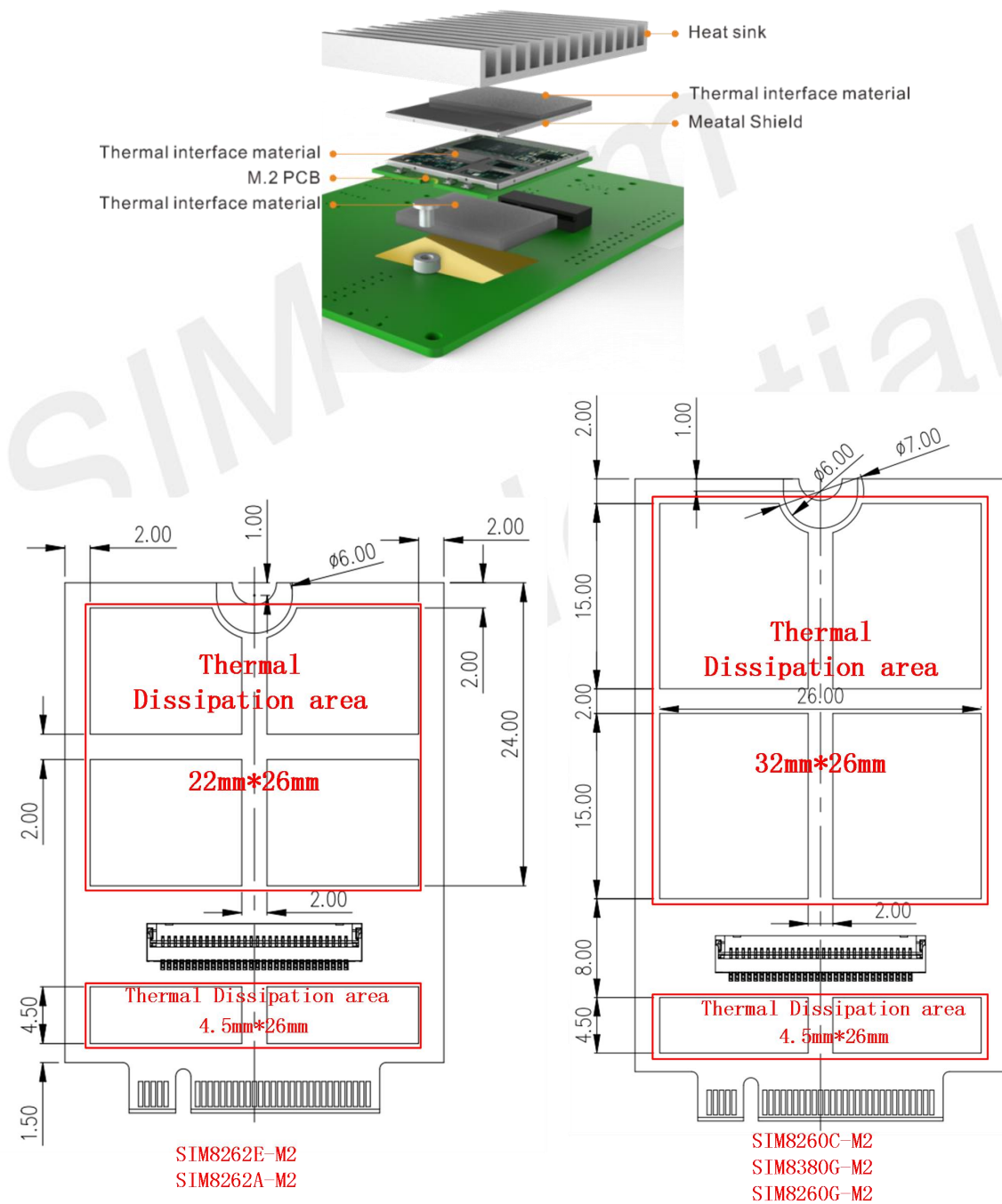
Figure 40: Thermal design diagram
