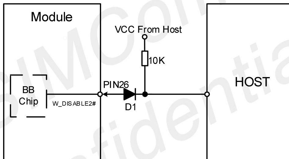
Figure 34: W_DISABLE2# pin reference circuit
