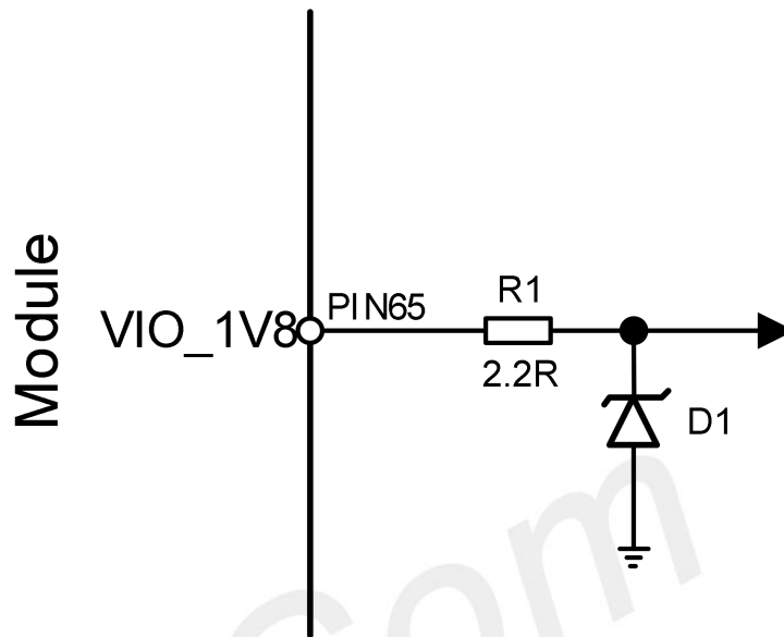
Figure 8: Power supply reference circuit
