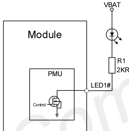
Figure 31: LED1# reference circuit
