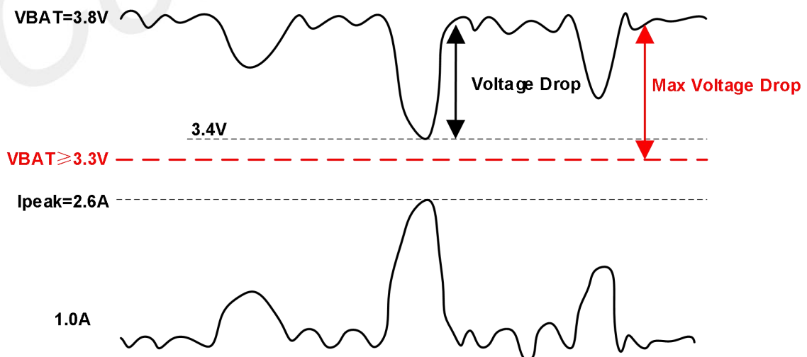
Figure 5: Power consumption of entire system
