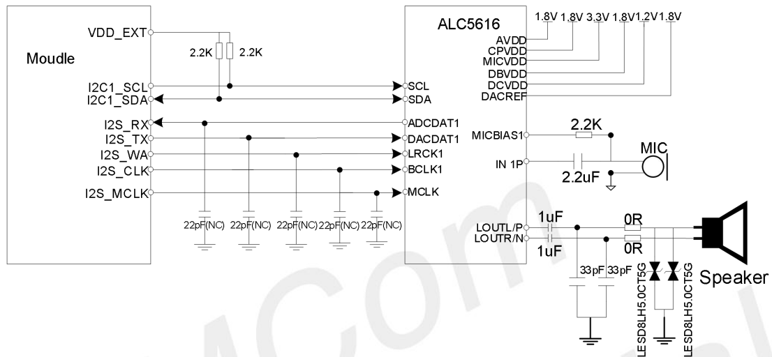
Figure 29: Audio codec reference circuit
