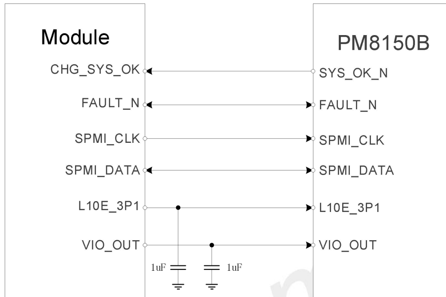
Figure 36: PM8150B interface diagram circuit
