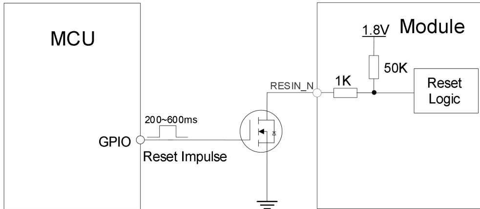
Figure 13: Reset the module use GPIO drive
