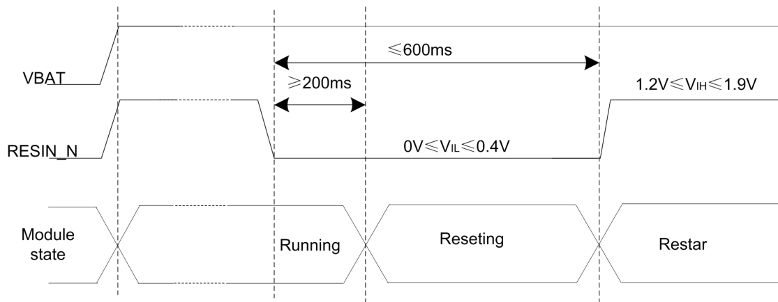
Figure 15: The reset timing sequence of the module
