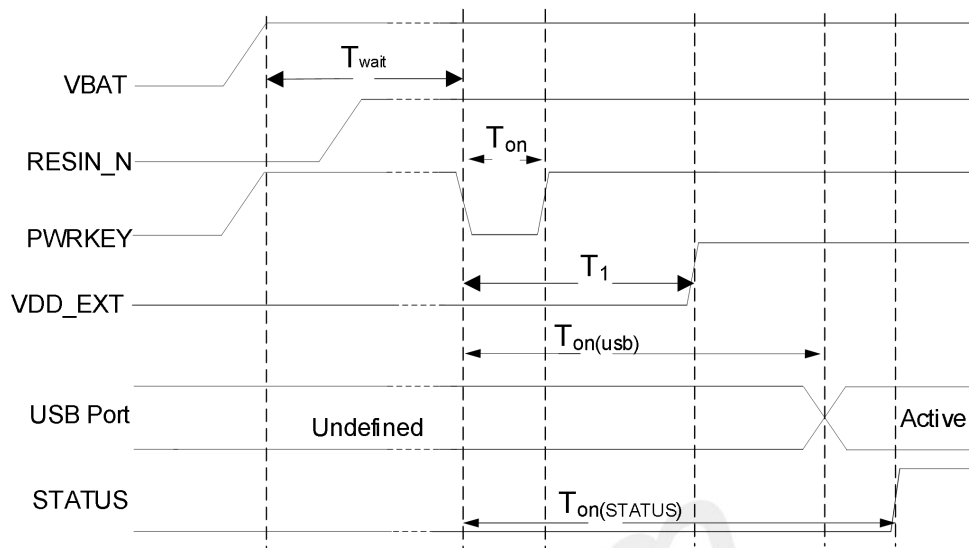
Figure 11: Power on sequence
