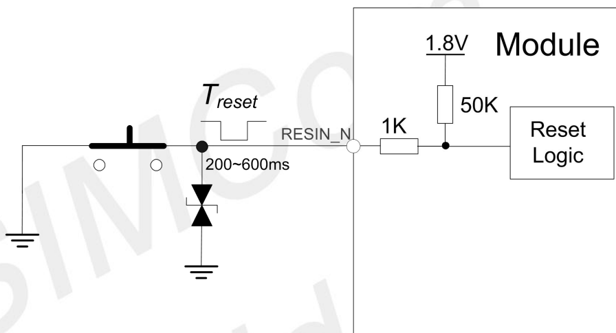
Figure 14: Reset the module use button
