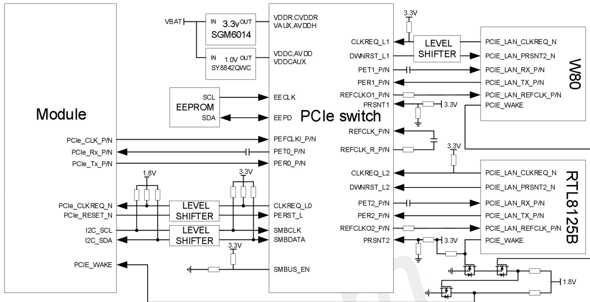
Figure 23: PCIe switch reference circuit
