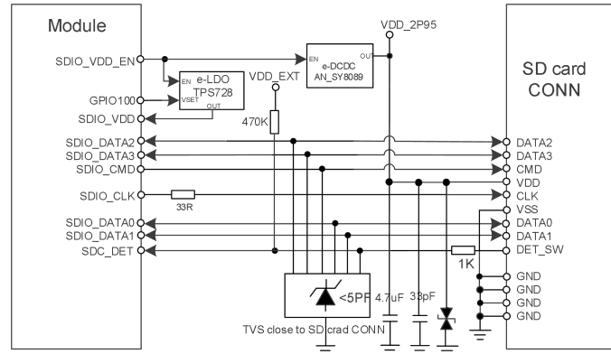
Figure 24: SD card reference circuit
