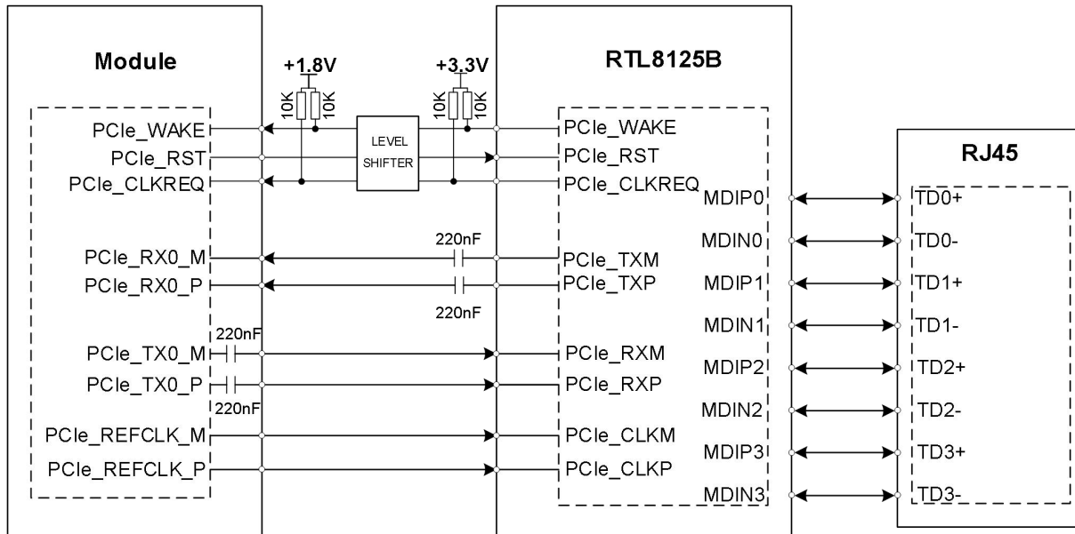
Figure 22: PCIe interface reference circuit (RC) for RTL8125B
