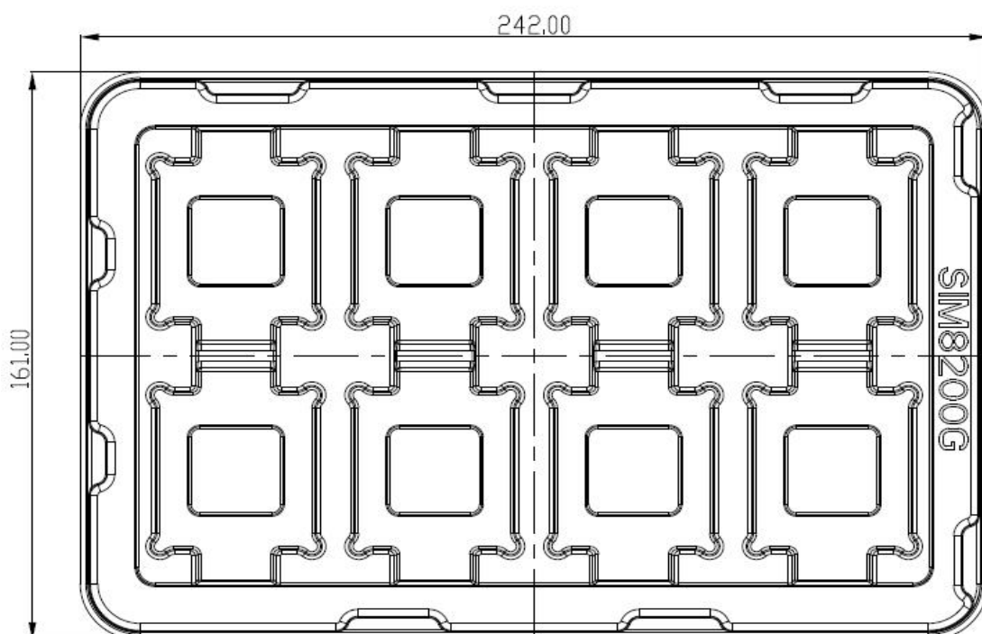
Figure 53: Module tray drawing
