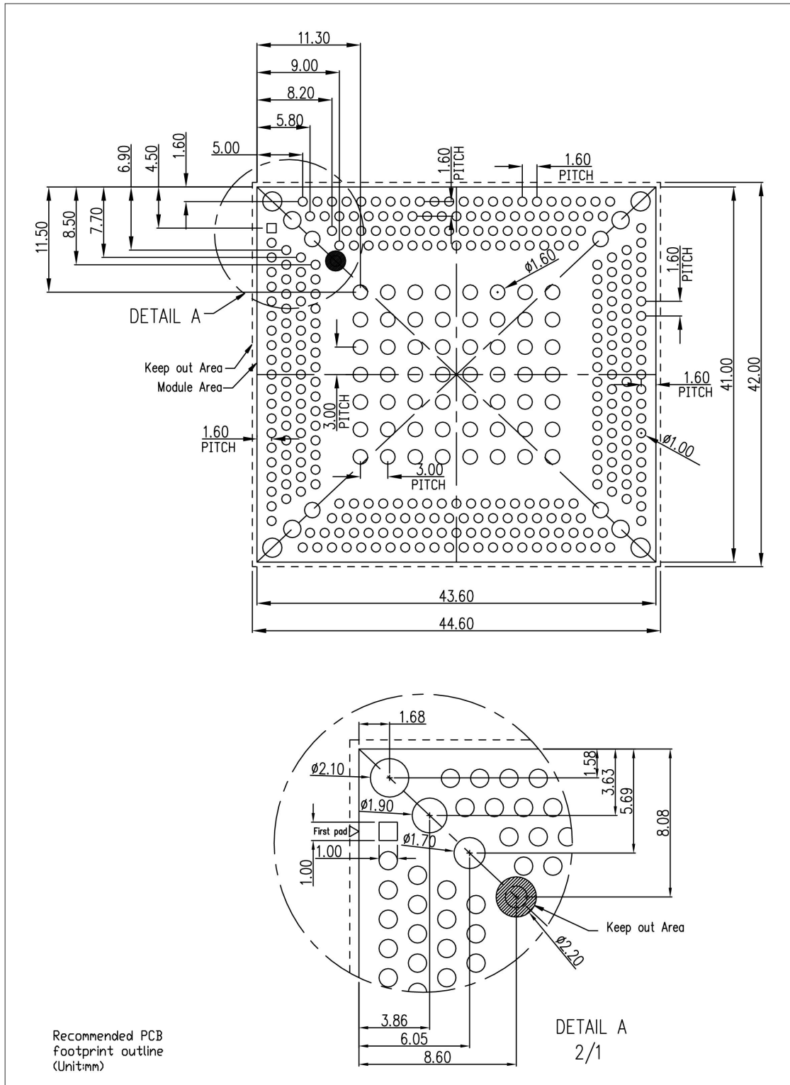
Figure 49: Recommended PCB footprint
