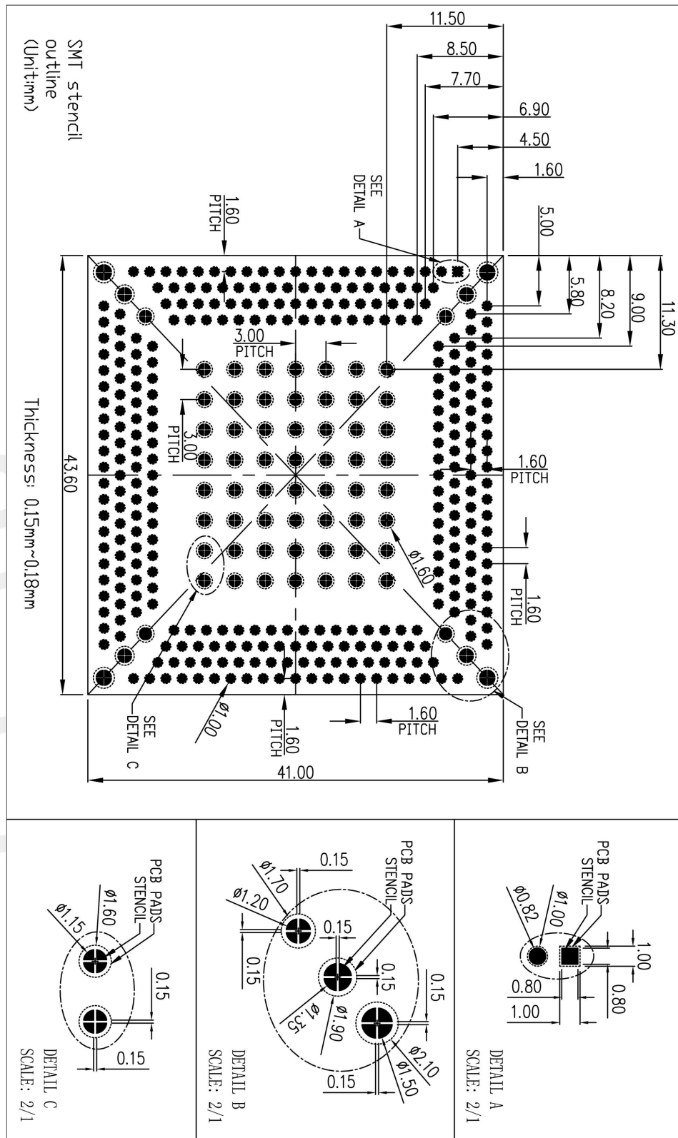
Figure 50: Recommended SMT stencil
