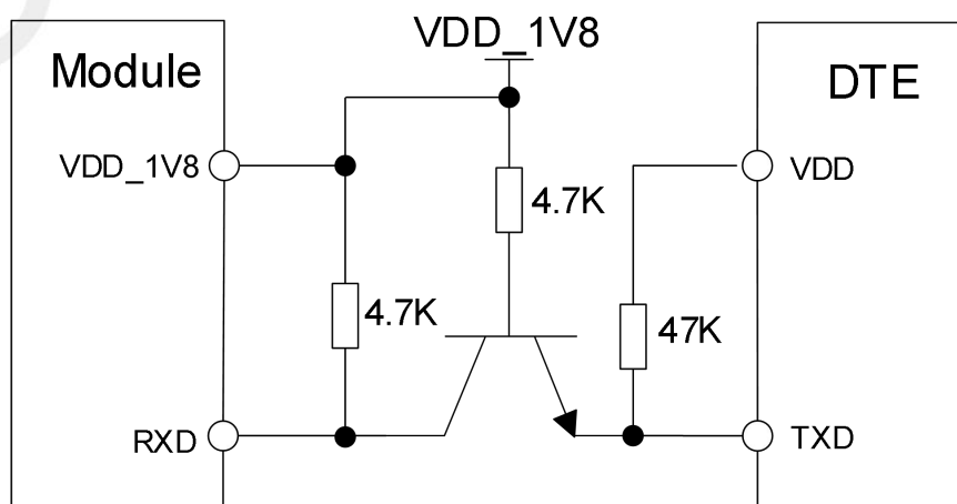
Figure 33: UART RX level conversion circuit
