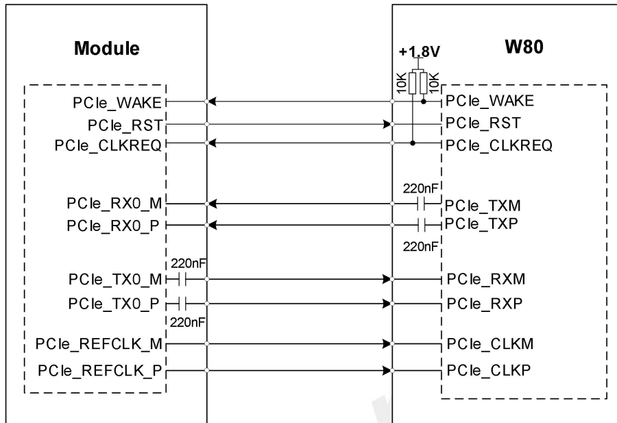
Figure 21: PCIe interface reference circuit (RC) for W80
