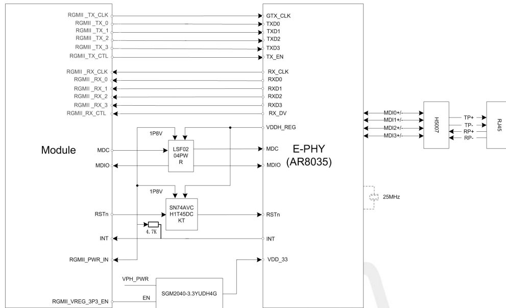
Figure 26: RGMII to RJ45 diagram circuit
