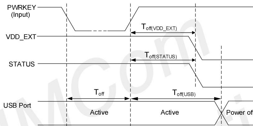
Figure 12: Power off sequence
