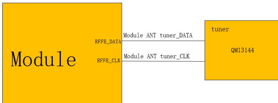
Figure 44: LGA package Tuner mipi interface
