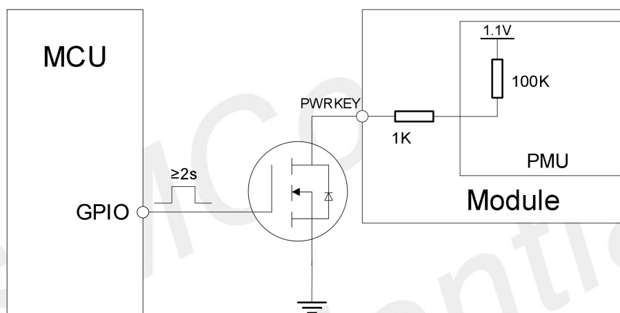
Figure 10: Power on the module use GPIO drive
