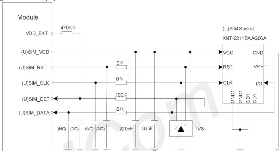
Figure 27: (U)SIM interface reference circuit
