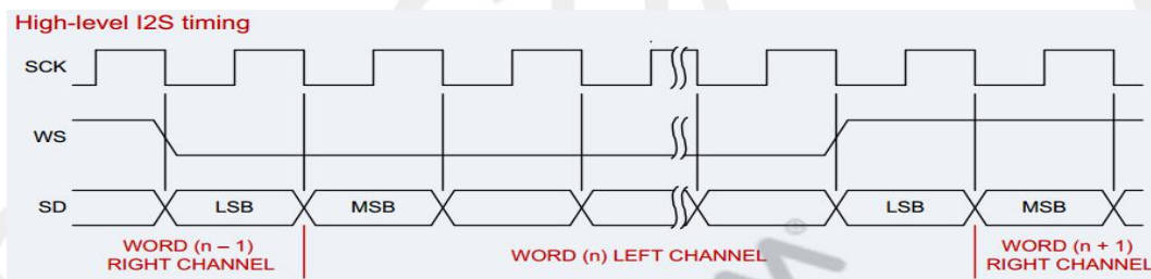
Figure 28: I2S timing
