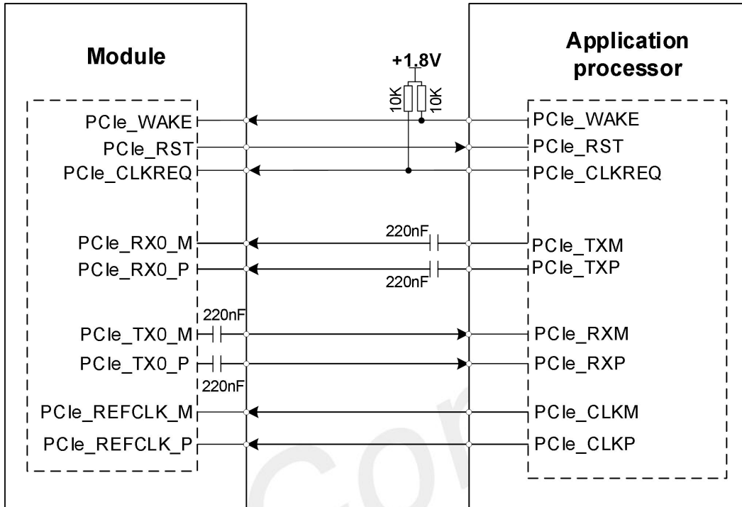
Figure 19: PCIe interface reference circuit (RC)
