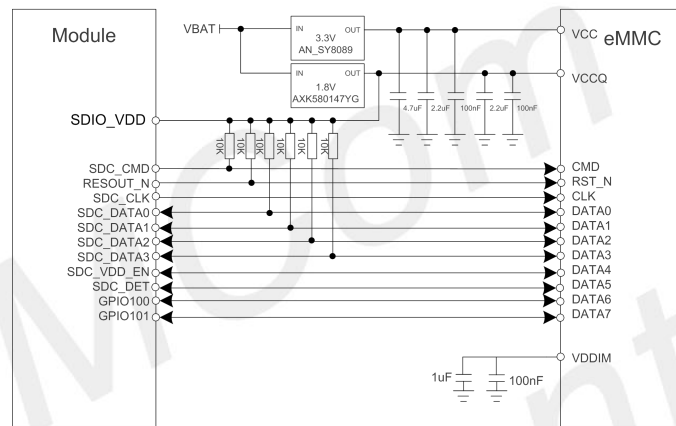
Figure 25: eMMC reference circuit
