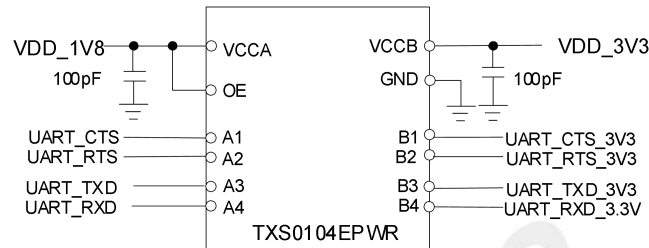
Figure 31: UART level conversion circuit
