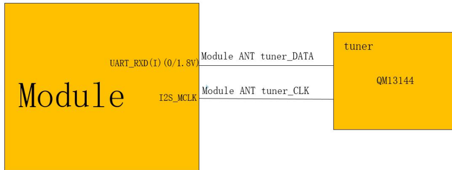
Figure 43: M.2 package Tuner mipi interface
