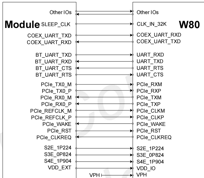
Figure 35: SIM8200G and W80 connect circuit
