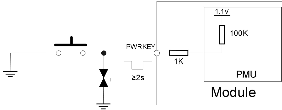
Figure 9: Power on the module use button
