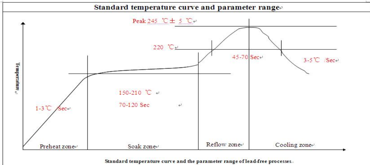
Figure 51: Recommended SMT reflow profile
