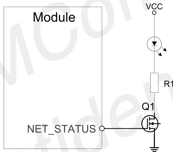
Figure 37: NET_STATUS reference circuit
