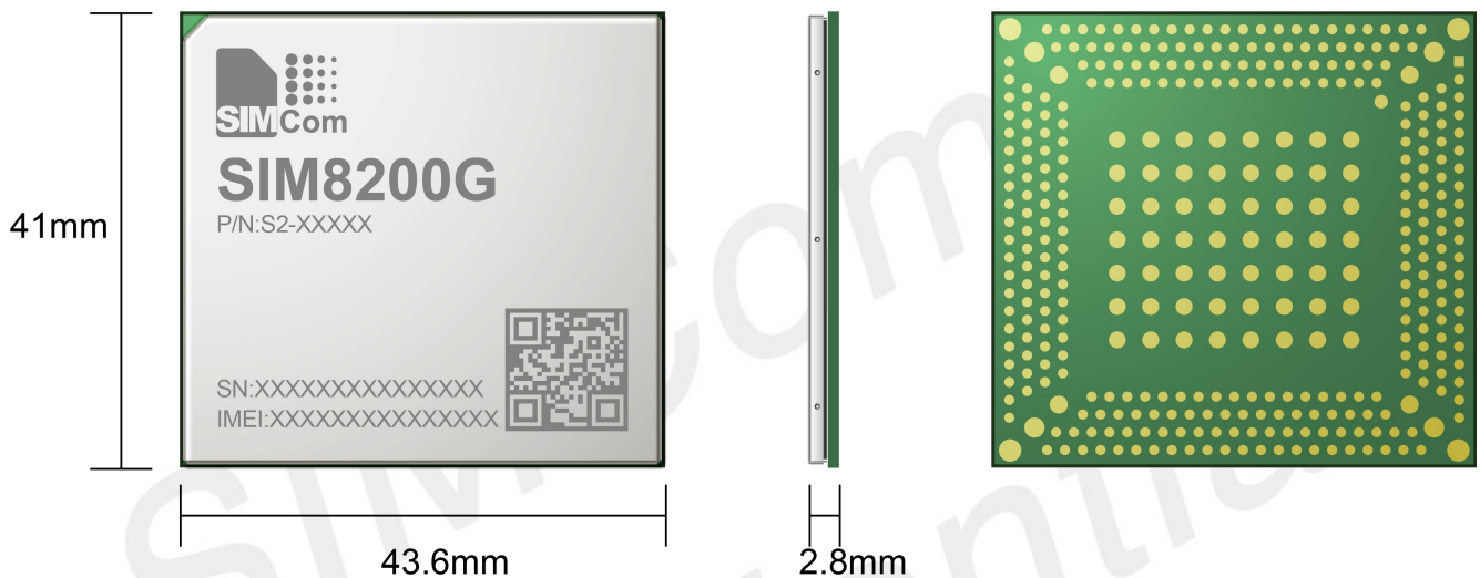
Figure 47: Top and bottom view of SIM8200G
