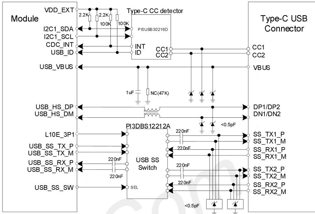
Figure 17: Type-C USB reference circuit with CC detector
