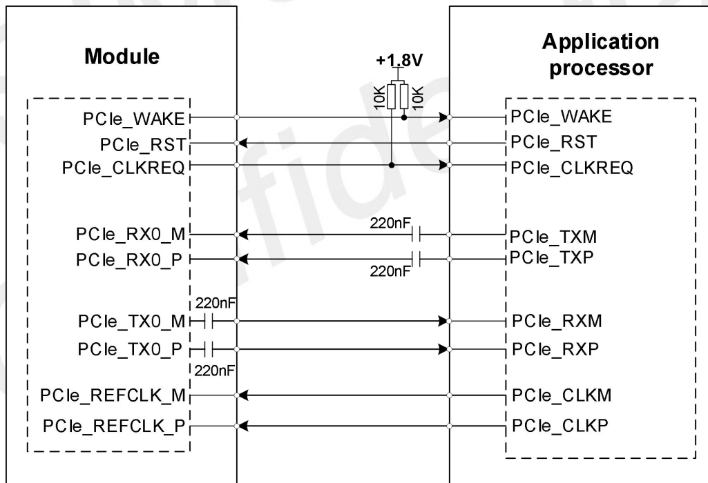
Figure 20: PCIe interface reference circuit (EP)
