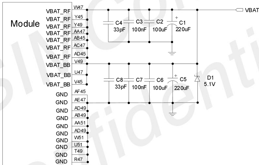
Figure 6: Power supply reference circuit
