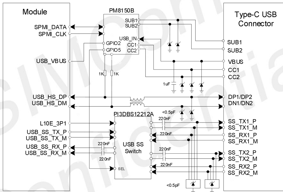
Figure 16: Type-C USB reference circuit with PM8150B
