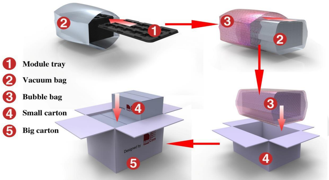
Figure 52: Packaging process
