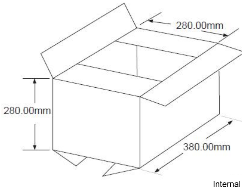
Figure 55: Big carton drawing
