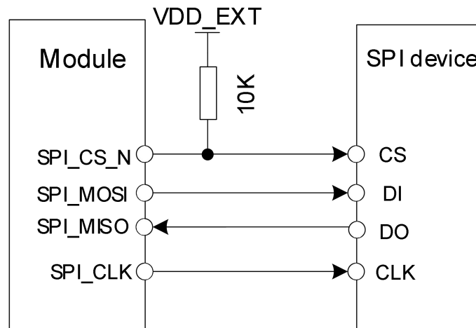
Figure 34: SPI reference circuit
