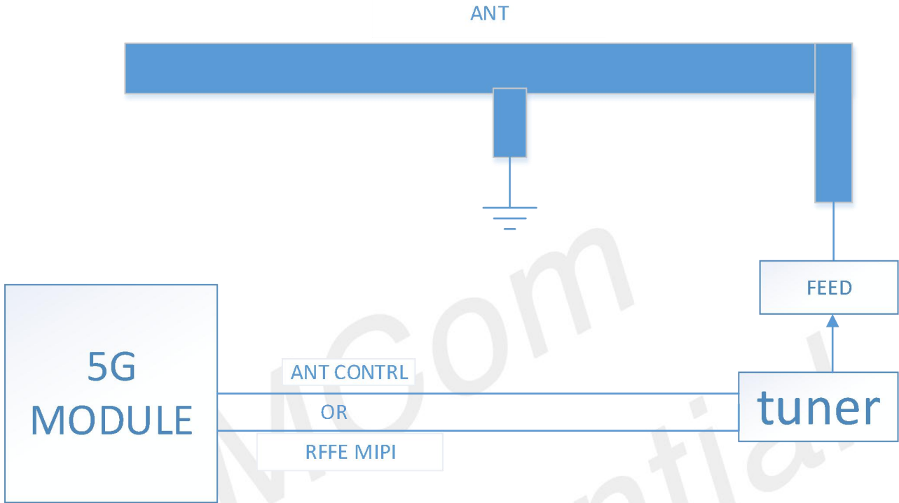
Figure 41: Impedance tuner reference block diagram
