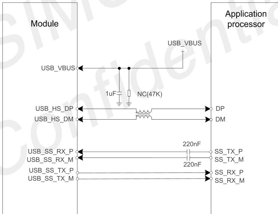
Figure 18: USB3.1 reference circuit
