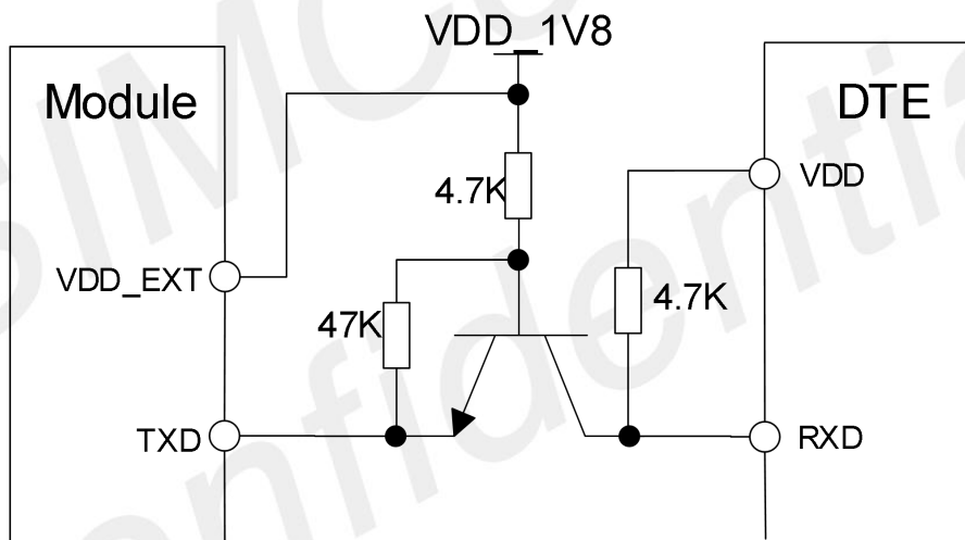
Figure 32: UART TX level conversion circuit
