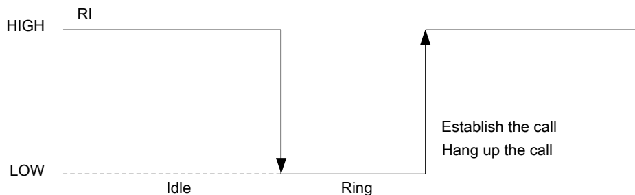
Figure 26: RI behaviour of voice calling as a receiver
