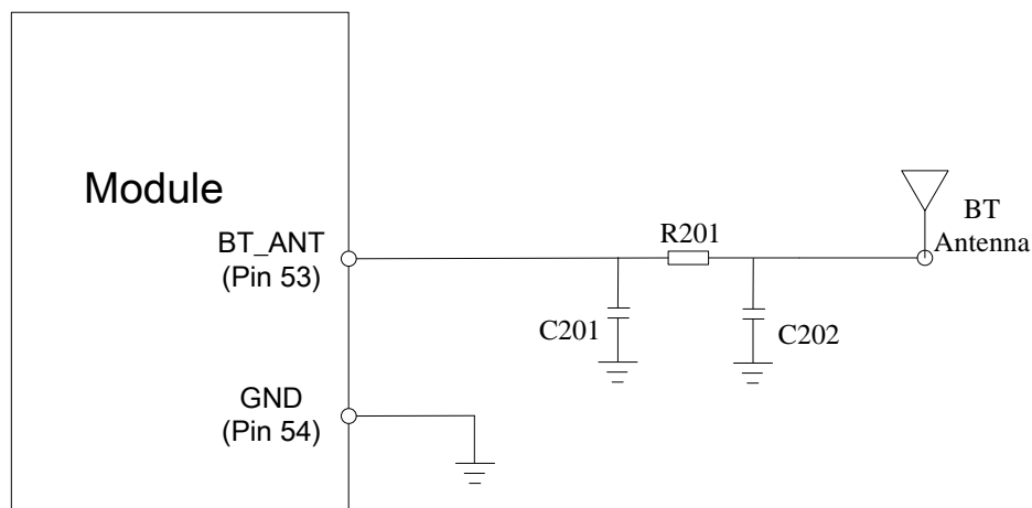
Figure 48: Bluetooth antenna matching circuit
