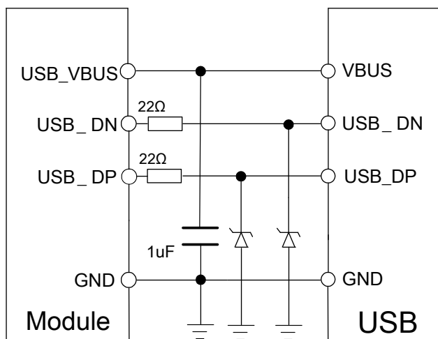
Figure 24: USB reference circuit
