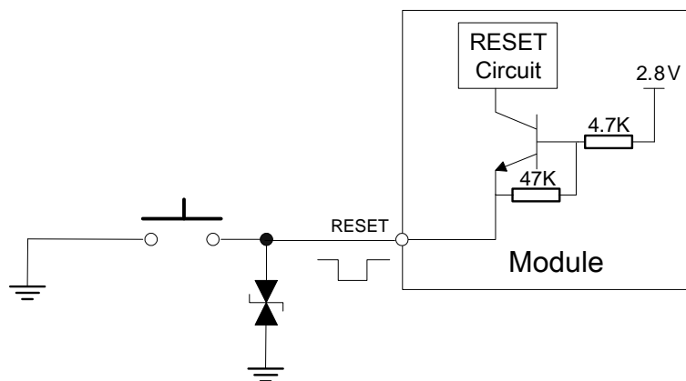
Figure 14: Reset circuit
