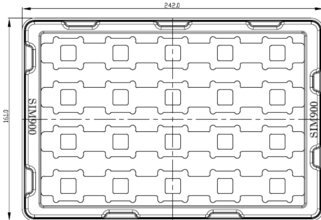
Figure 53: Tray drawing
