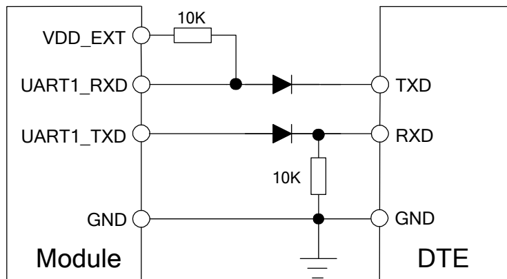
Figure 21: Isolation circuit by diodes
