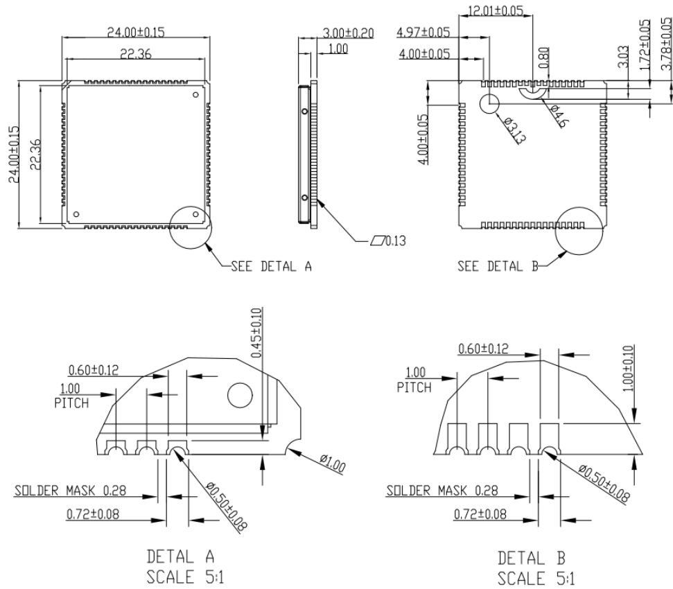
Figure 3: Dimensions of SIM800 (Unit: mm)
