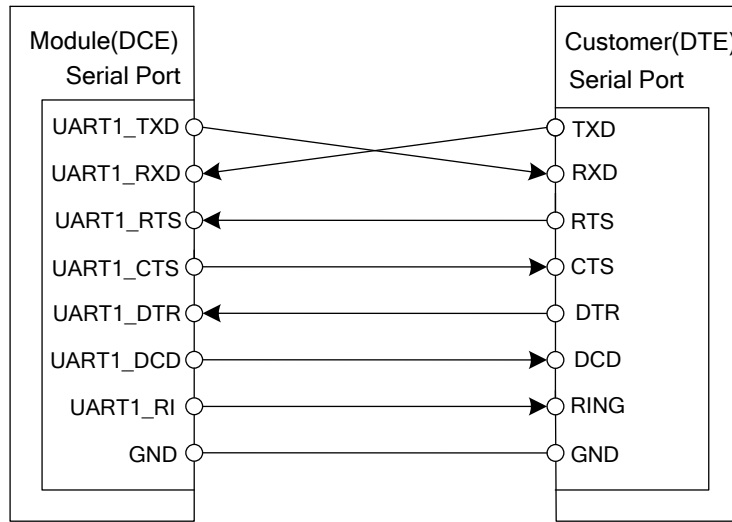
Figure 19: Connection of the serial port
