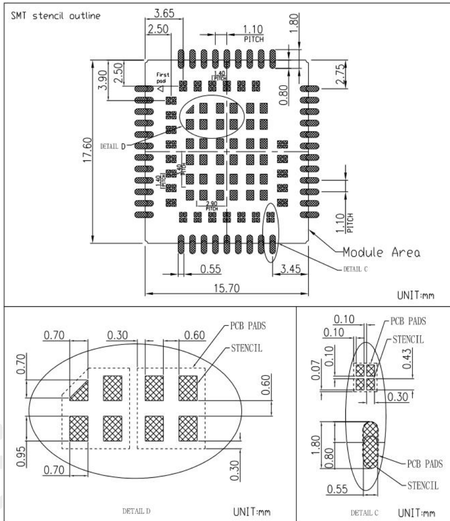
Figure 36: stencil recommendation (Unit: mm)
