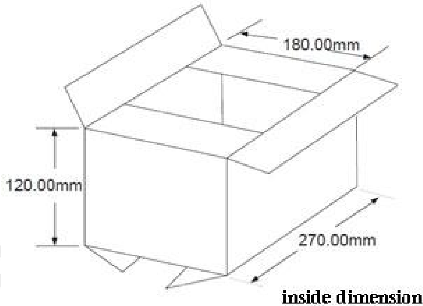
Figure 39: Small carton drawing
