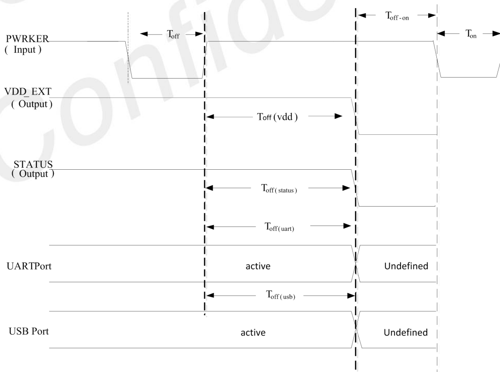
Figure 9: Power off timing sequence
