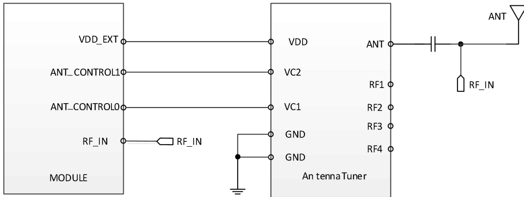
Figure 26: RFGRFC interface reference circuit
