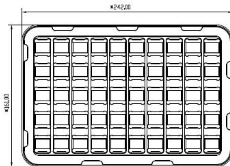
Figure 38: Tray drawing
