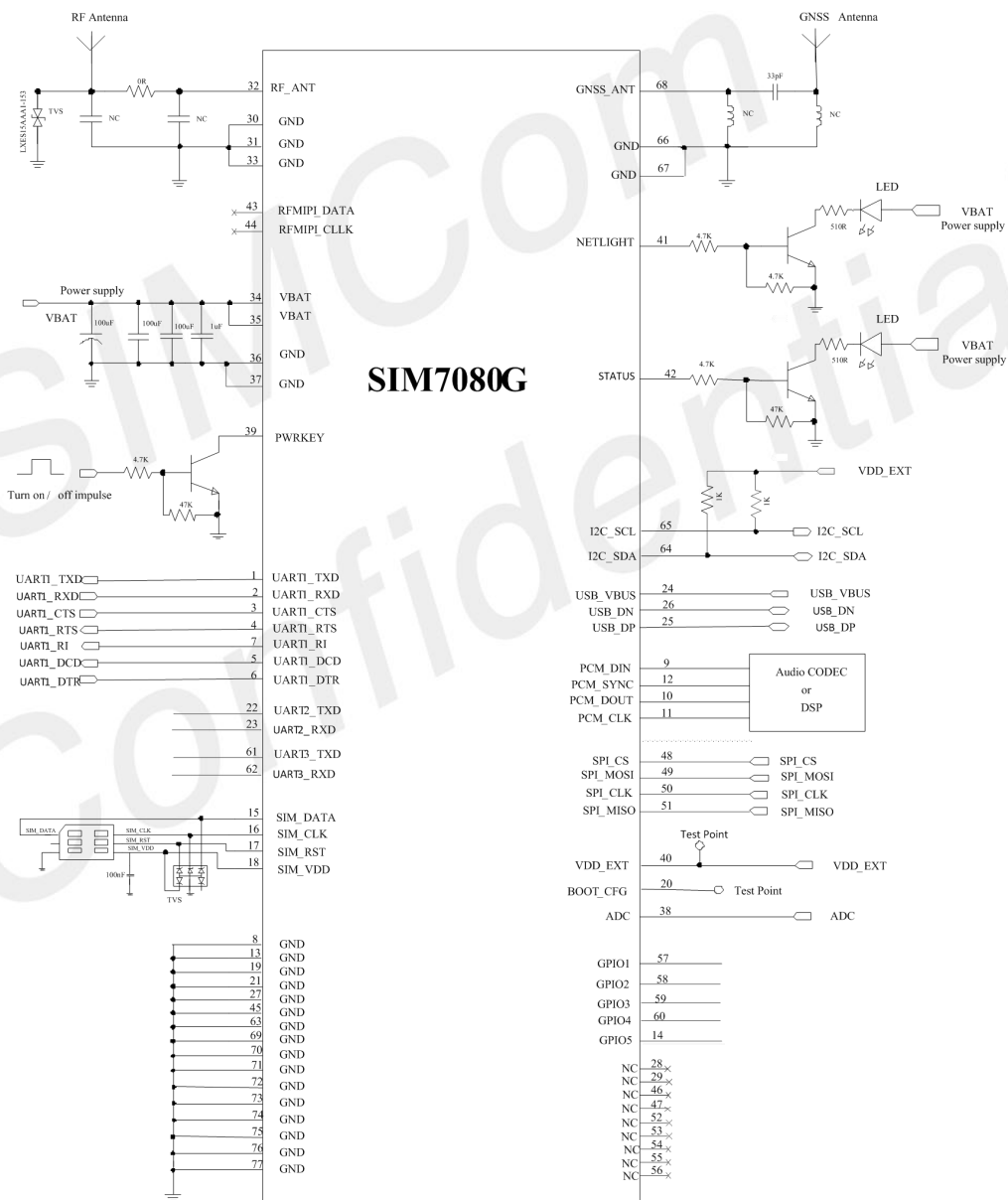
Figure 41: Reference design
