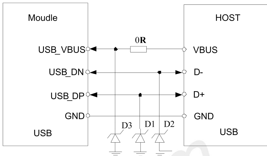
Figure 15: USB reference circuit
