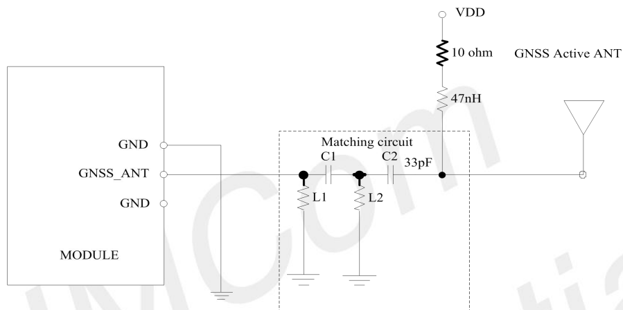
Figure 28: Active antenna circuit
