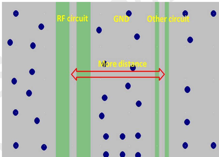
Figure 30: RF trace should be far away from other high speed signal lines
