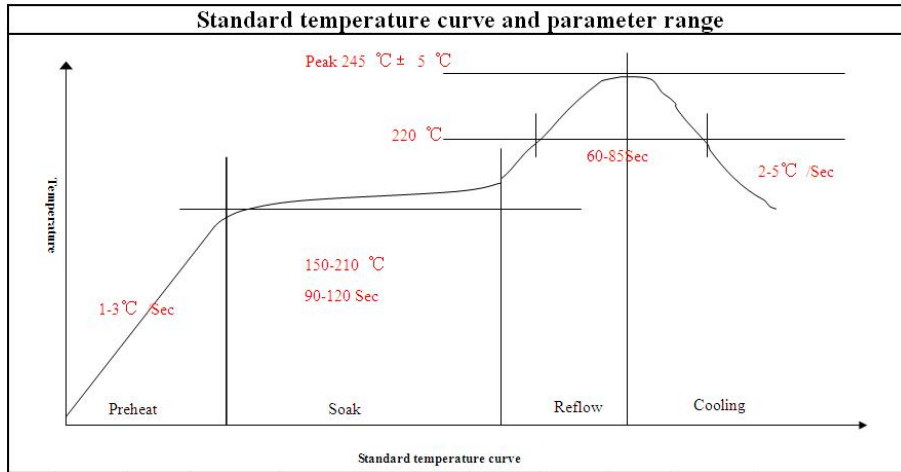
Figure 35: The ramp-soak-spike reflow profile of SIM7080G
