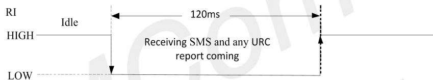
Figure 14: RI behaviour (SMS and URC report)
