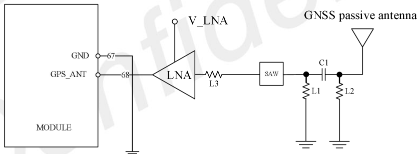
Figure 29: Passive antenna circuit (Default)
