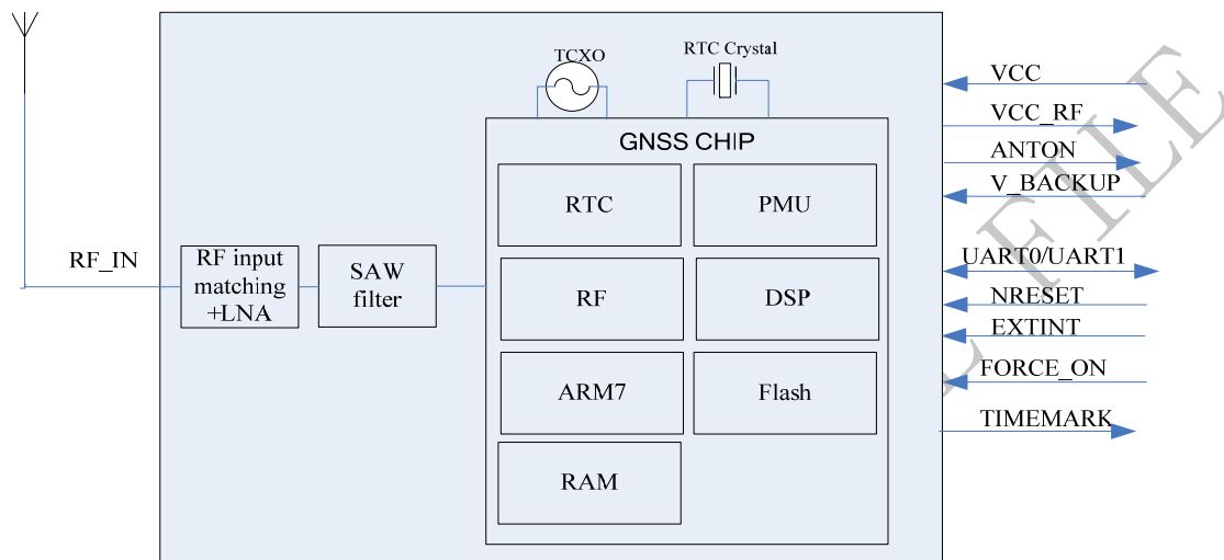
Figure 1: SIM68M functional diagram
