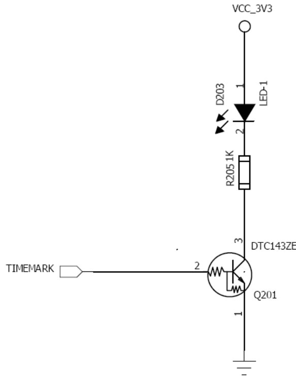
Figure 6: TIMEMARK application circuit
