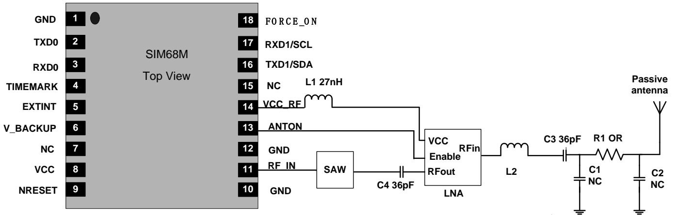
Figure 8: SIM68M passive antenna design (with external LNA and SAW)
