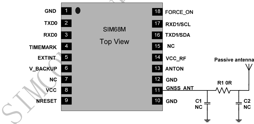
Figure 7: SIM68M passive antenna design
