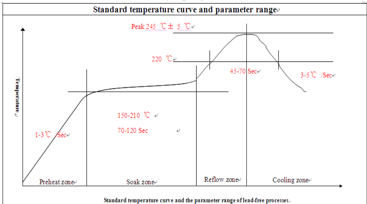
Figure 13: The Ramp-Soak-Spike reflow profile of SIM68M
