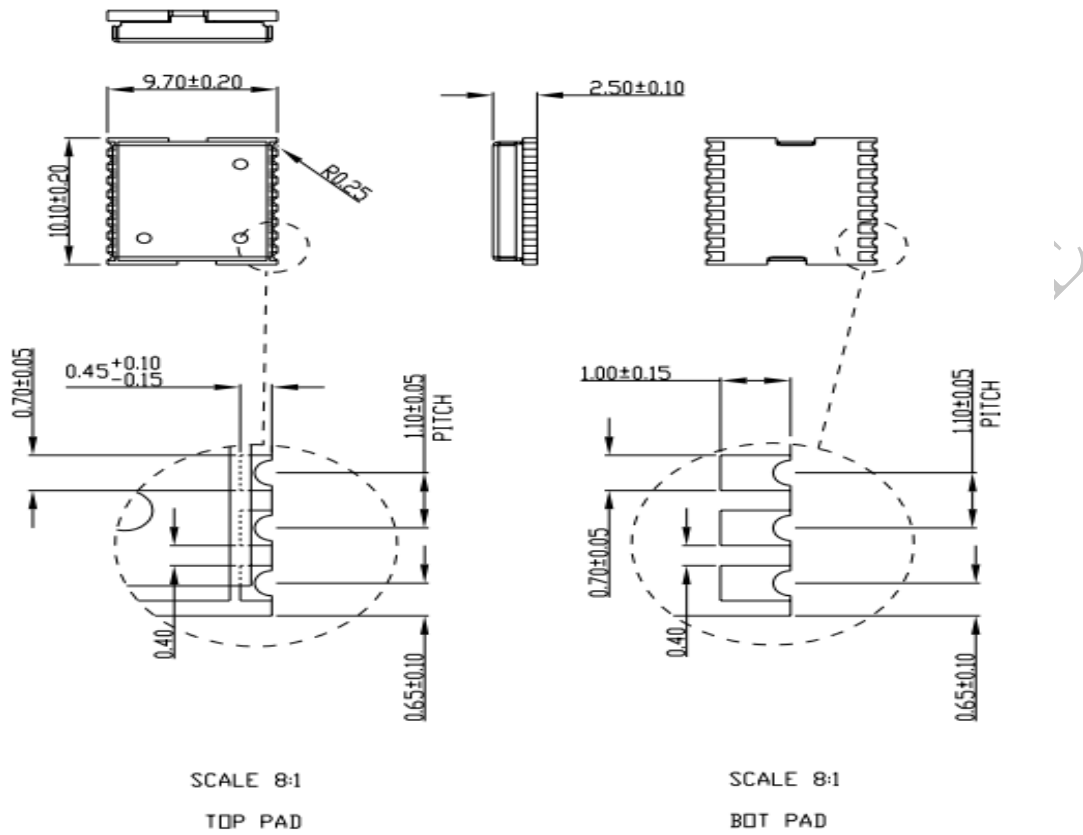
Figure 3: SIM68M mechanical dimensions (Unit: mm)
