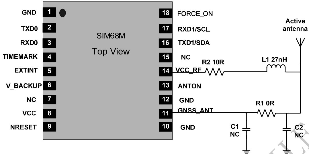
Figure 10: SIM68M Active antenna design
