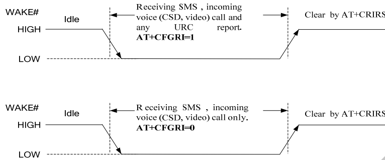
Figure 7: WAKE# behaviour
