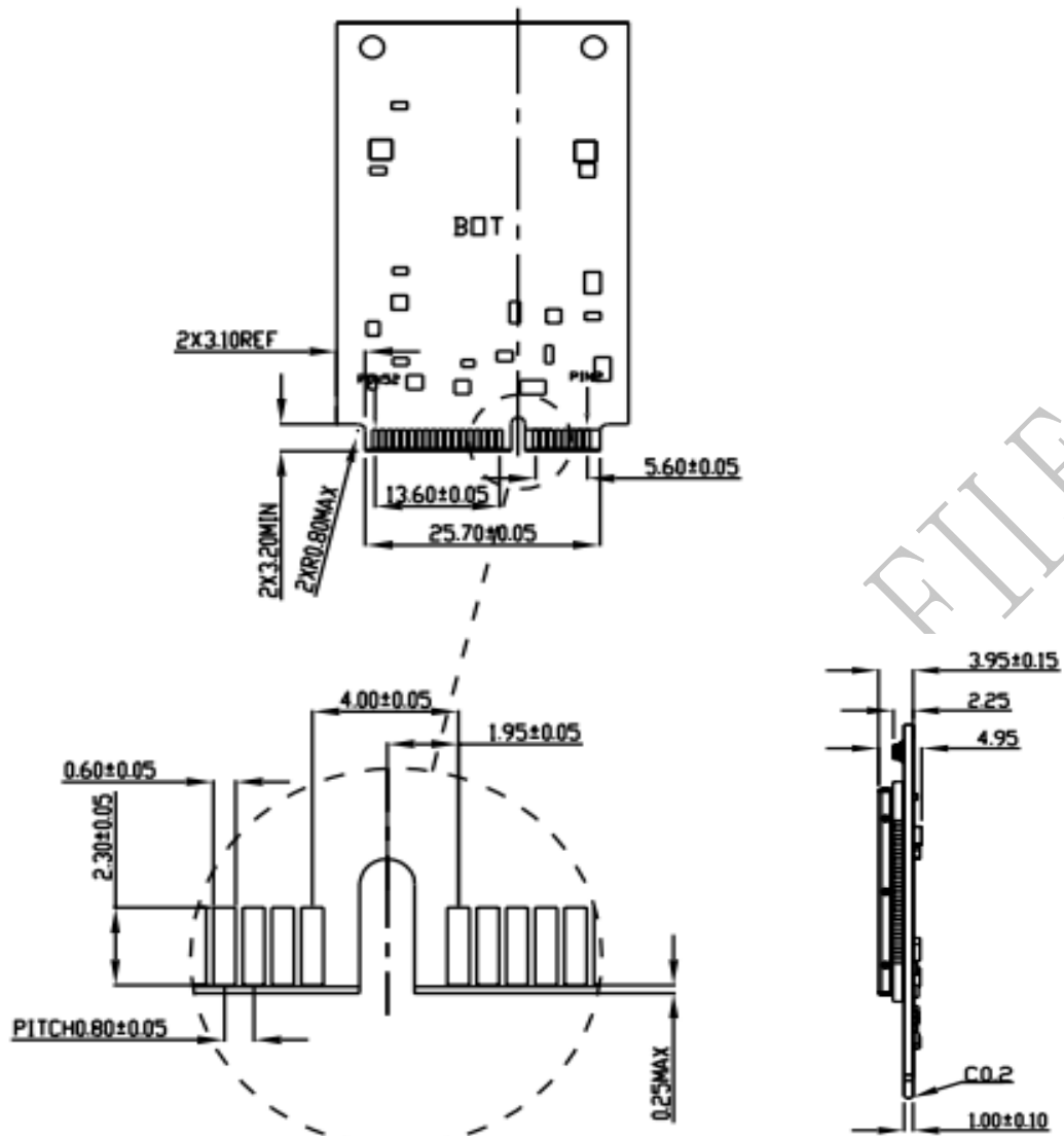
Figure 12: Dimensions of SIM5360-PCIE (Unit: mm Bottom and Side view)
