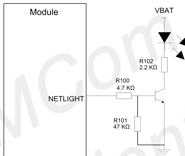
Figure 33: NETLIGHT Reference Circuit
