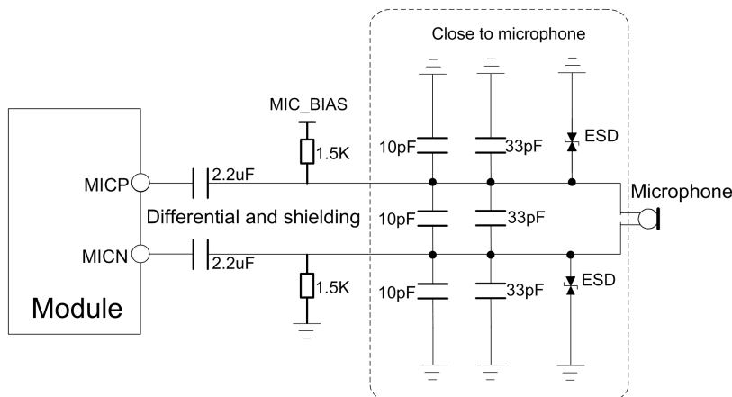
Figure 23: Microphone Circuit
