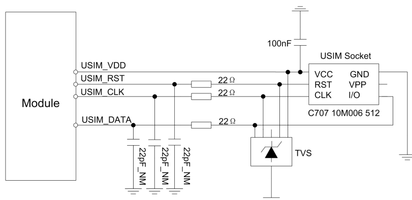
Figure 24: USIM Interface Reference Circuit
