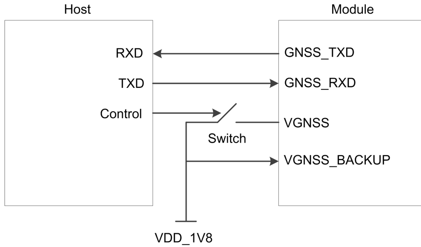
Figure 35: GNSS Circuit Diagram (NMEA to host UART)
