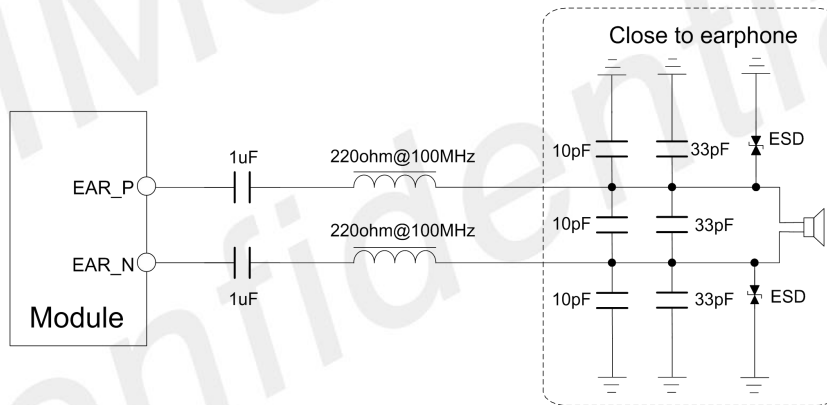
Figure 22: Receiver Circuit
