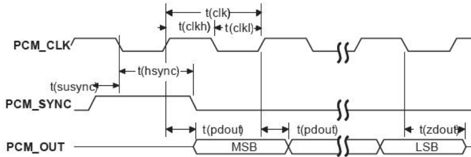
Figure 29: Module to Codec Timing
