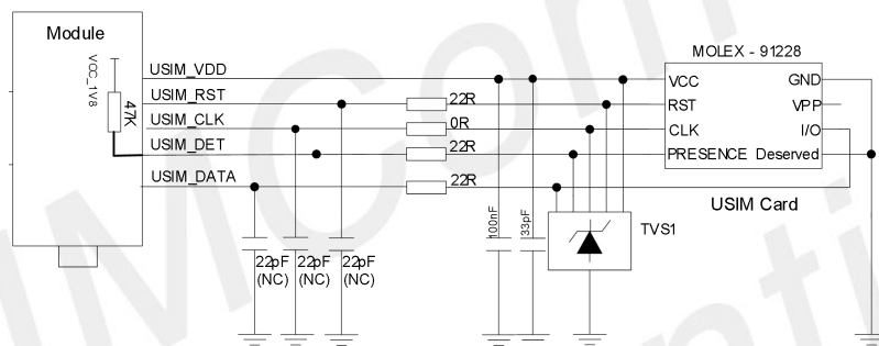
Figure 25: USIM Interface Reference Circuit with USIM_DET
