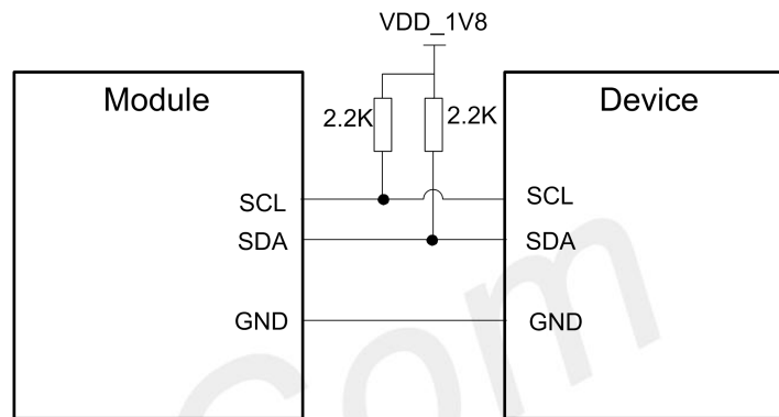
Figure 32: I2C Reference Circuit
