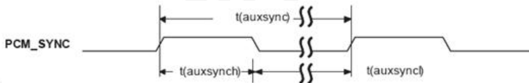
Figure 27: PCM_SYNC Timing
