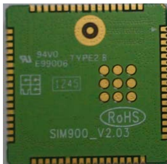
PCB Version 1245
