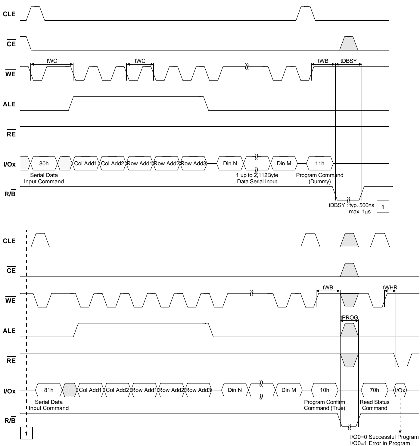
Ex.) Two-Plane Page Program
