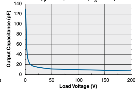
Output Capacitance vs. Load Voltage ( I_F=5\text{mA} , f=1\text{MHz} , T_A=25^\circ\text{C} )
