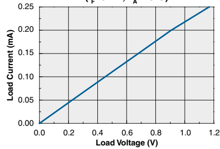
Typical Load Current vs. Load Voltage DC-Only Configuration ( I_F=0\text{mA} , T_A=25^\circ\text{C} )
