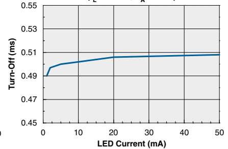
Typical Turn-Off vs. LED Forward Current ( I_L=70\text{mA} , T_A=25^\circ\text{C} )
