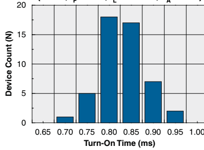
Typical Turn-On Time (N=50, I_F=5\text{mA} , I_L=130\text{mA} , T_A=25^\circ\text{C} )
