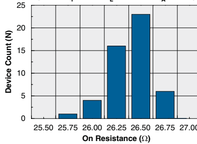
Typical On-Resistance Distribution (N=50, I_F=2\text{mA} , I_L=130\text{mA} , T_A=25^\circ\text{C} )
