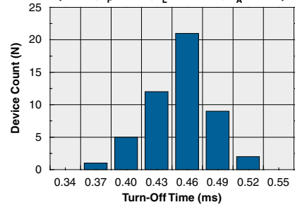
Typical Turn-Off Time (N=50, I_F=5\text{mA} , I_L=130\text{mA} , T_A=25^\circ\text{C} )
