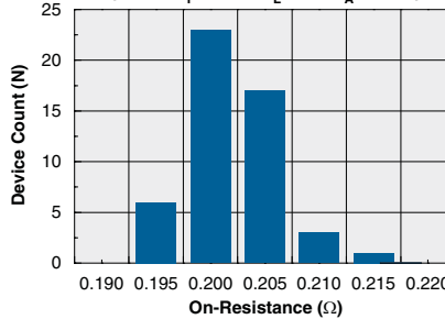
Typical On-Resistance Distribution (N=50, I_F=2\text{mA} , I_L=1\text{A} , T_A=25^\circ\text{C} )
