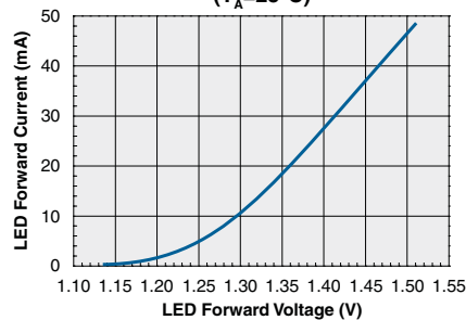
LED Forward Voltage vs. LED Forward Current ( T_A=25^\circ\text{C} )
