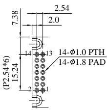
PIN DETAIL
