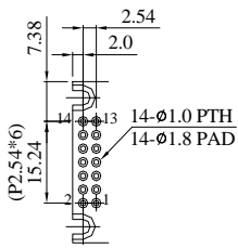
PIN DETAIL
