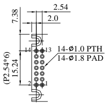
PIN DETAIL
