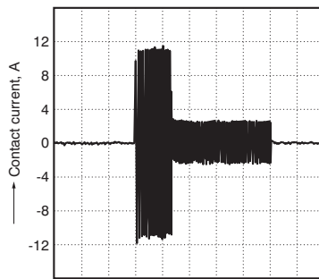
Inrush current wave form vs time
