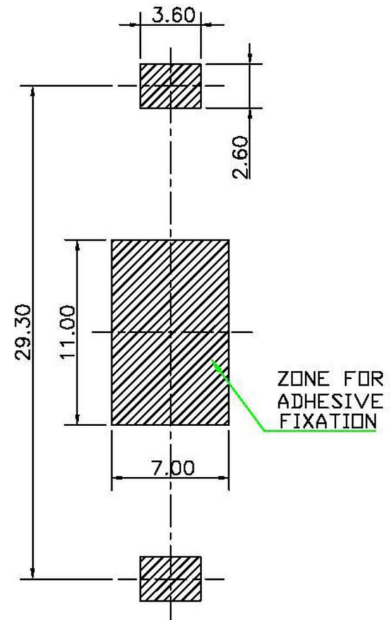
PCB LAYOUT
