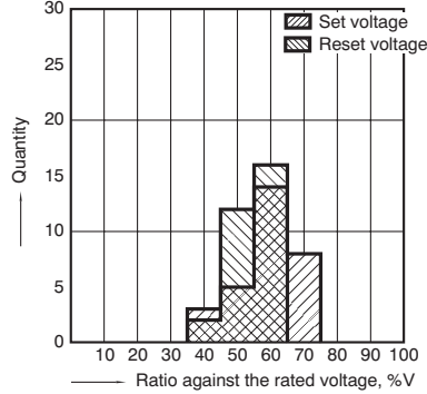
8. Distribution of set and reset voltage
