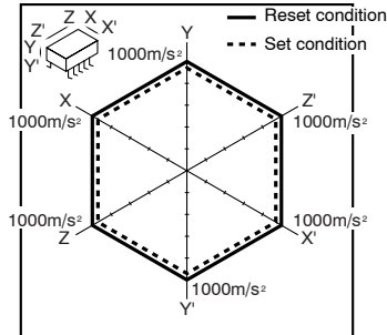
12.-(2) Malfunctional shock (latching)
