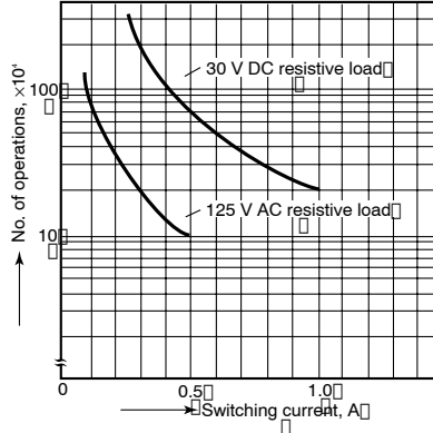
2. Life curve
