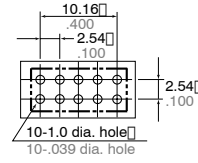
PC board pattern (Copper-side view)
