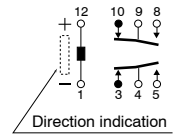
1 coil latching (Reset condition)
