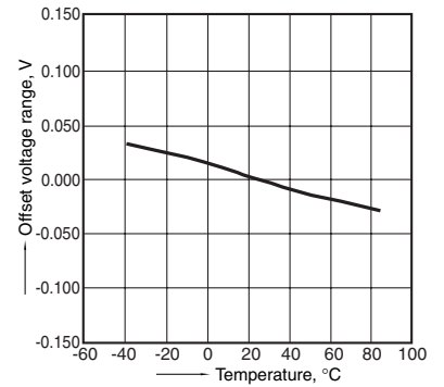
3. Offset voltage temperature characteristics (Typical value)
