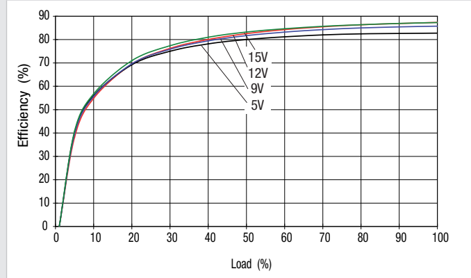
NMK 5V Input Voltage
